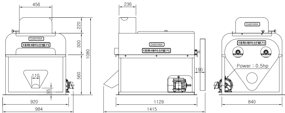
Broken Rice Separator (Middle)
