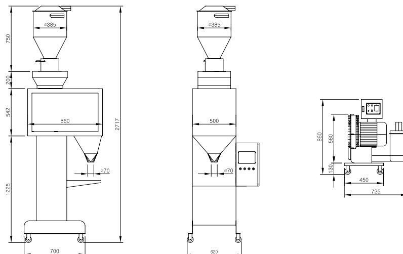
Auto Measuring / Packing Machine (DPS-1 & Vacuum transfer device)
