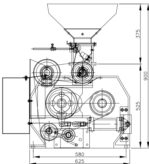
Rice Huller (MJH-SBCA)
