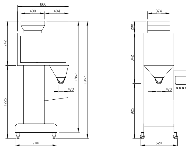
Auto Measuring / Packing Machine (DPS-1)
