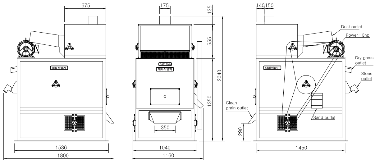
Comprehensive Stone Separator Dolsoe(45B)
