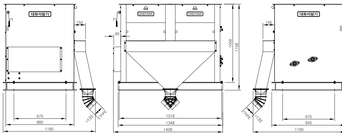
Stone Separator Dolsoe(Double)
