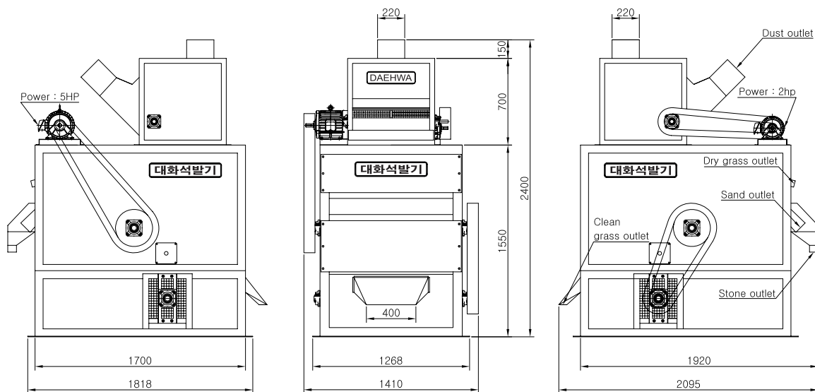
Comprehensive Stone Separator Dolsoe(60B)
