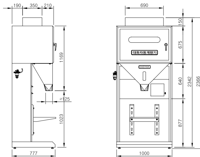
Automatic Weighing Machine (HK-2000)
