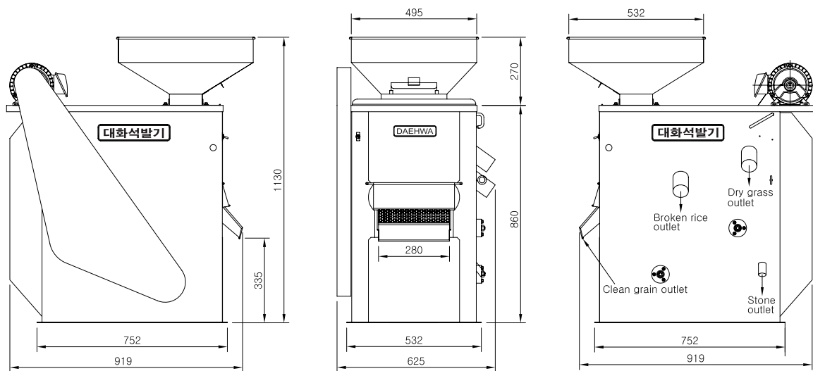
Stone Separator Dolsoe(Home use)
