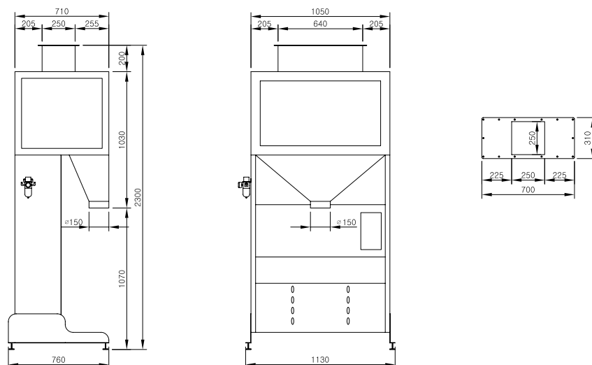
Automatic Weighing Machine(DP-2)
