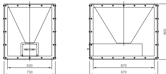
A Support for the stone separator
