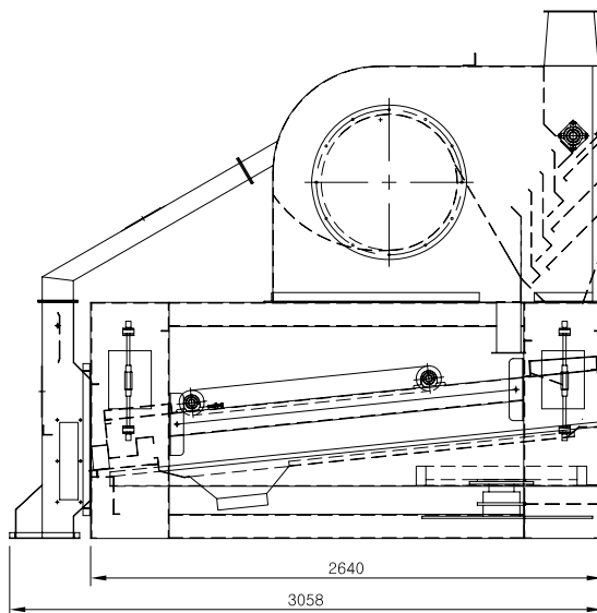
Pre Cleaner (SS4019)
