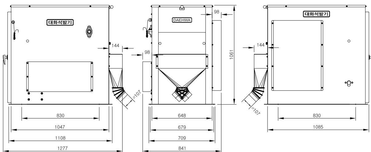
Stone Separator Dolsoe II(Single)
