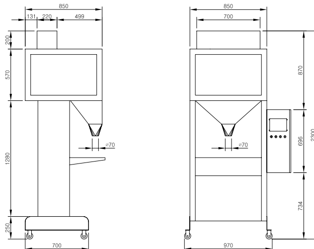
Auto Measuring / Packing Machine (DPS-2)
