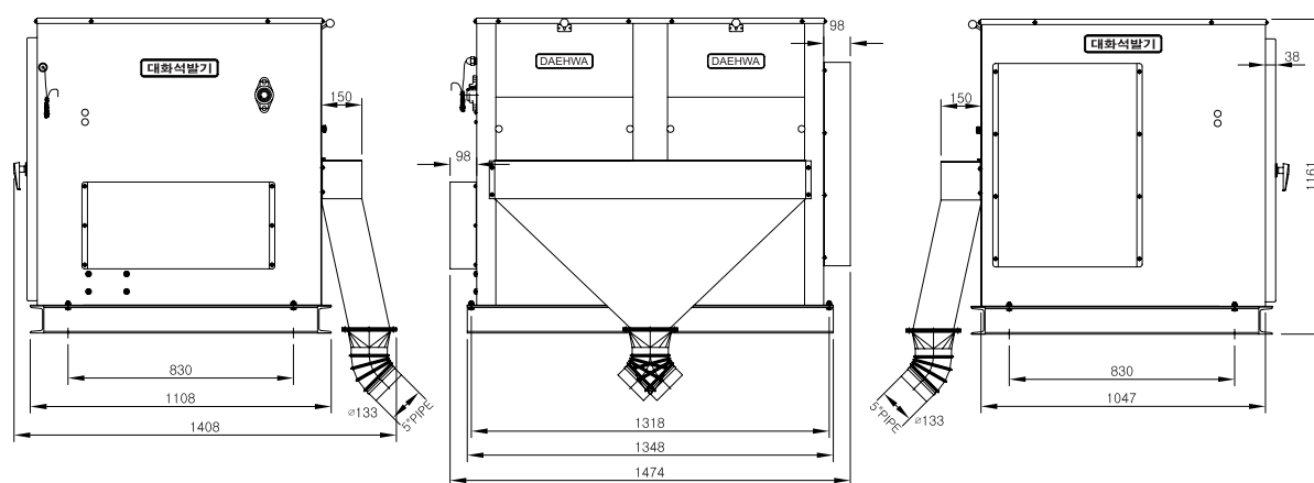
Stone Separator Dolsoe II (Double)
