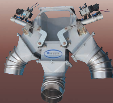
Auto 3-way gate
