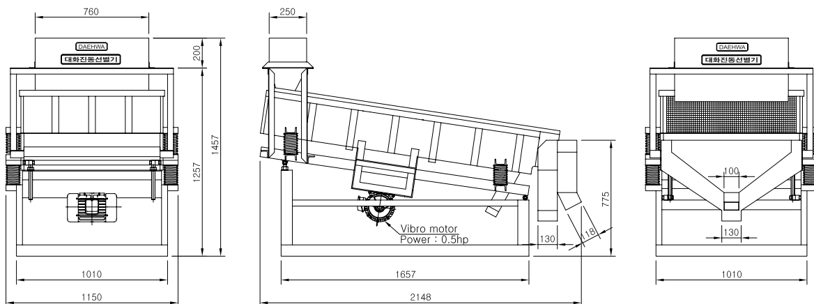
Vibratory Separator (Middle)
