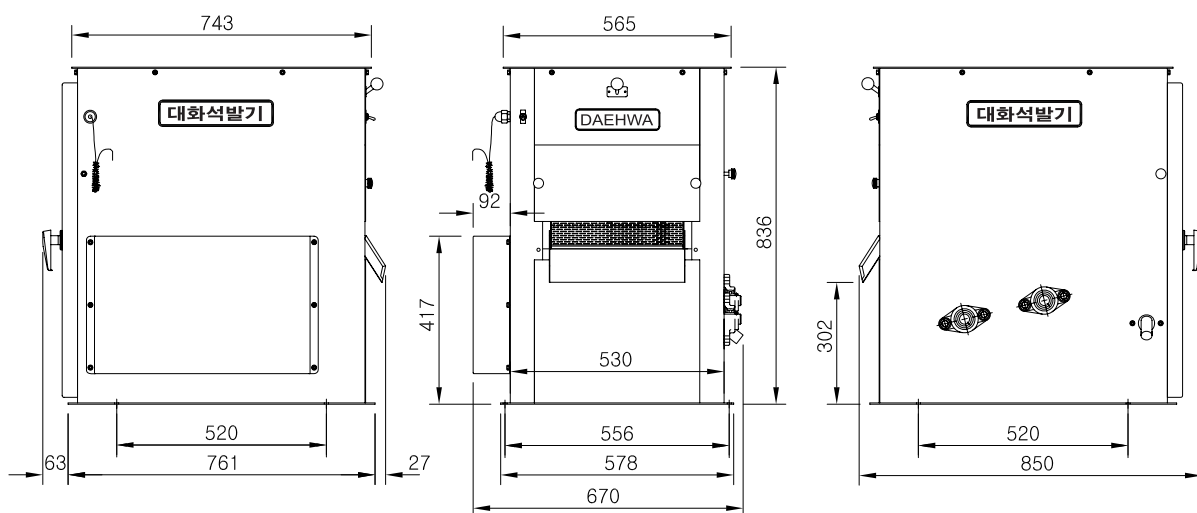
Stone Separator Dolsoe(Small)
