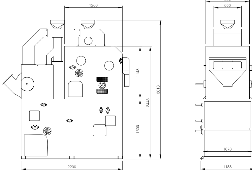
Comprehensive Stone Separator Dolsoe(ISPC-60)
