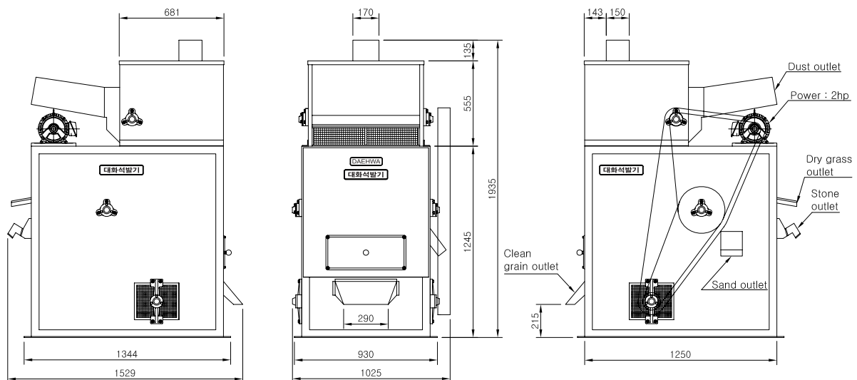
Comprehensive Stone Separator Dolsoe(40B)
