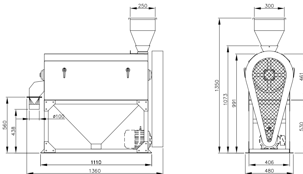
Green-Kerneled Rice Separator (SS30)
