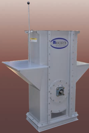
Lower section for Bucket Elevator
